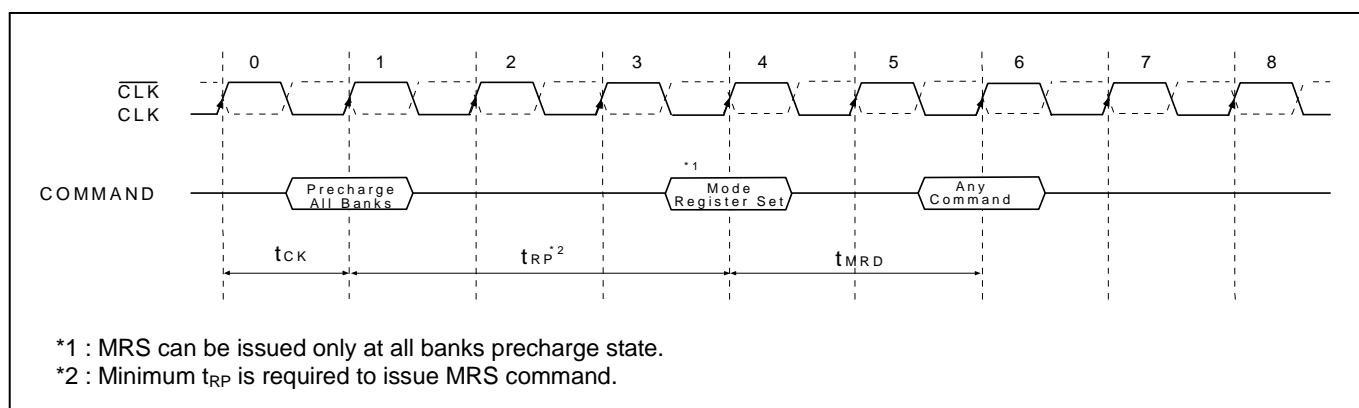
Mode Register Set
